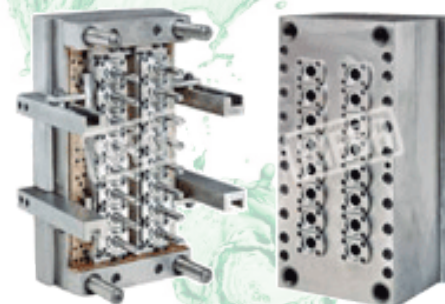
MOULD FOR PCO 1810 NECK FINISH
