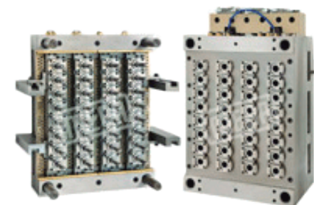
MOULD FOR 38MM NECK FINISH
